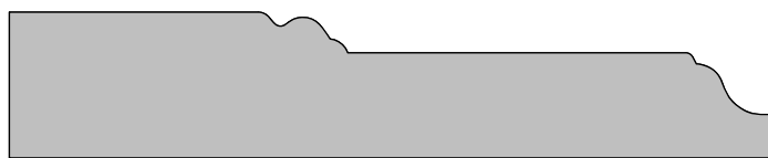
3 5/8" x 11/16" #12-167
